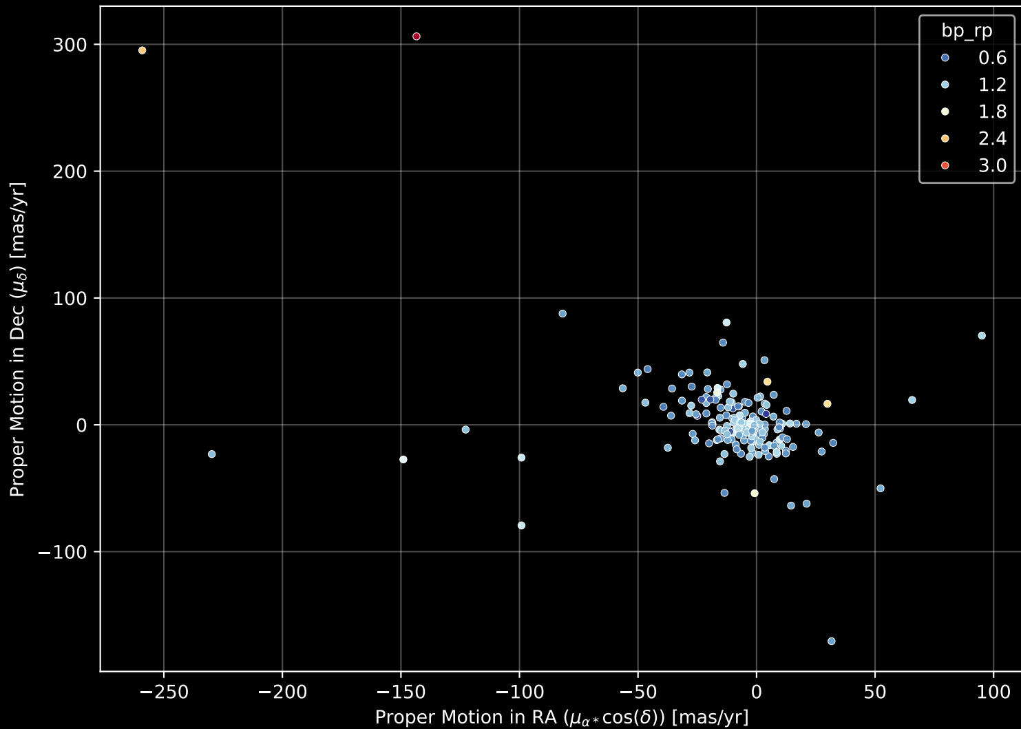
APOGEE DR17 Field: [065+43_MGA] Proper Motion Diagram (n= 184)
